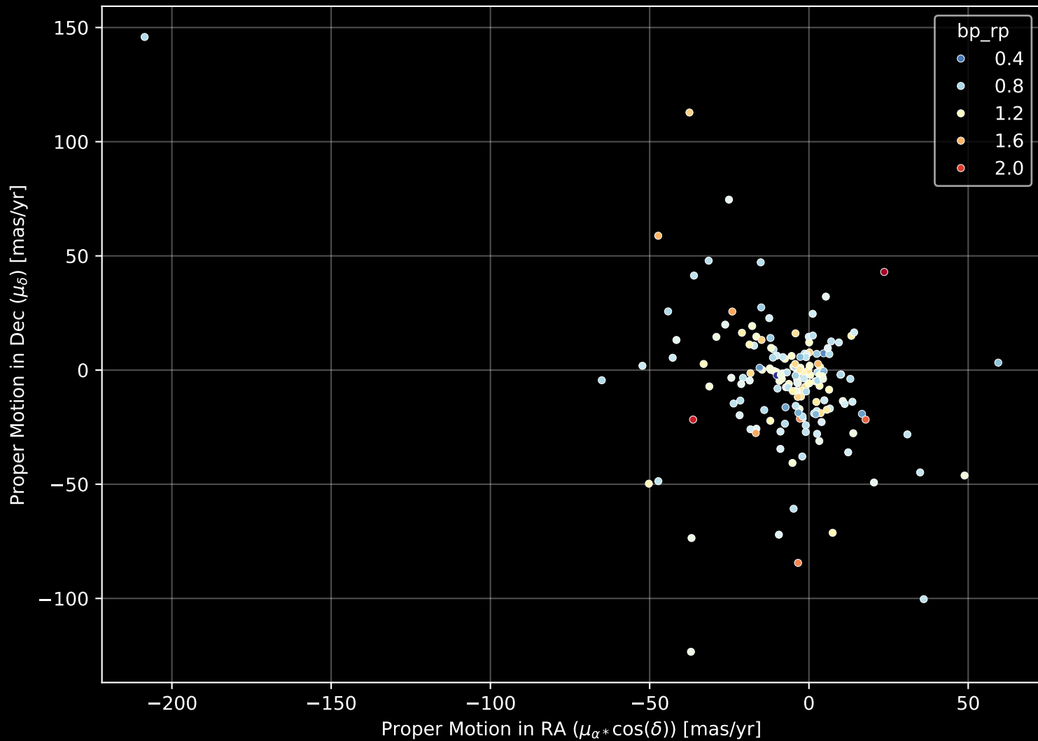
APOGEE DR17 Field: [047+39_MGA] Proper Motion Diagram (n= 170)
