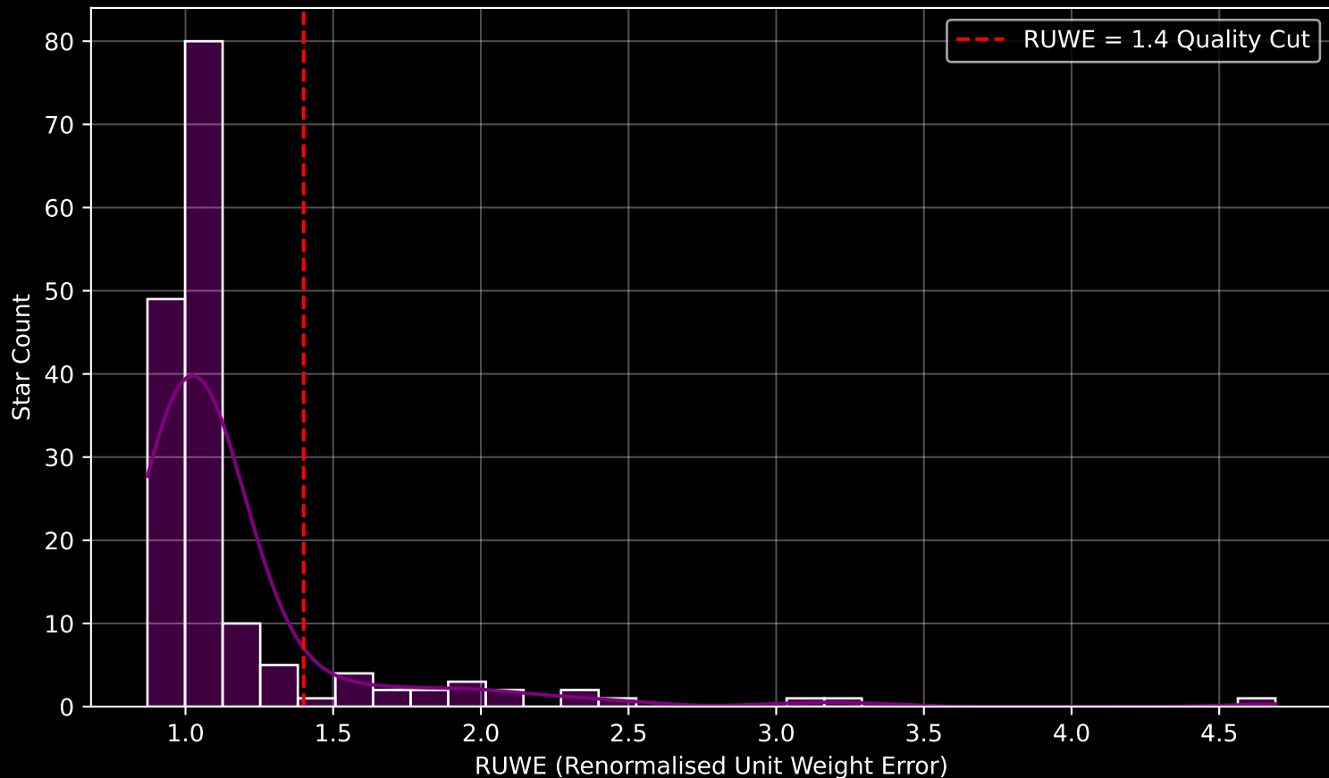
GAPOGEE DR17 Field [047+39_MGA] RUWE Distribution (n= 164)
