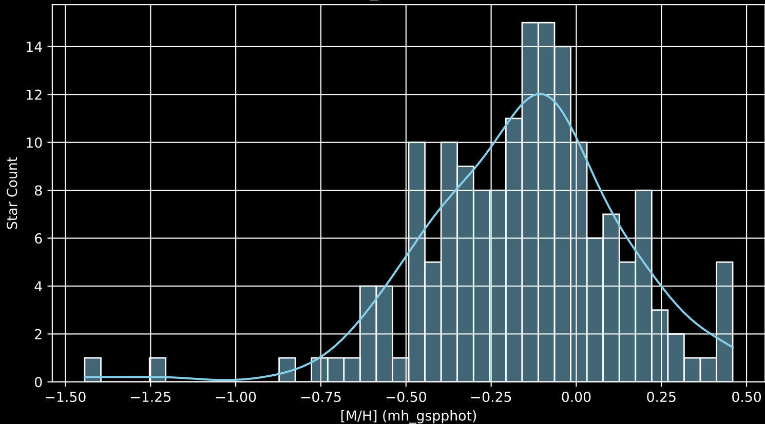
APOGEE DR17 Field: [047+39_MGA [M/H] (mh_gspphot) (n= 168)
