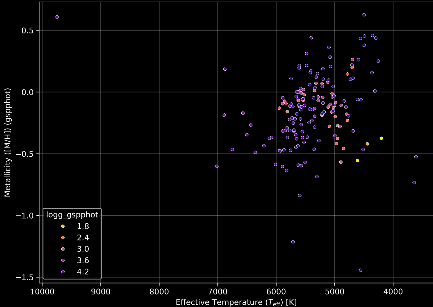
APOGEE DR17 Field: [047+39_MGA] Stellar Population Parameters (n= 170)
