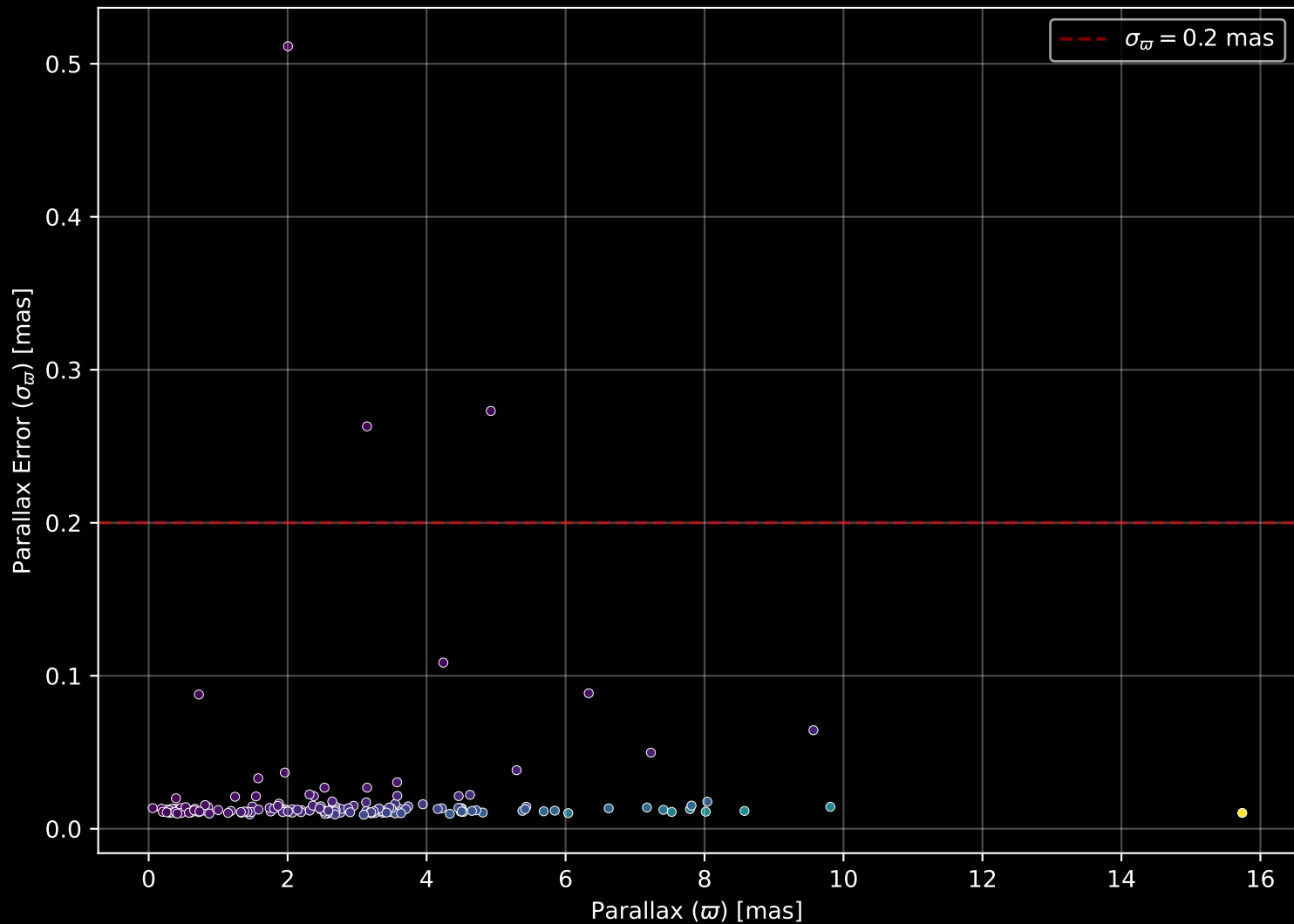
APOGEE DR17 Field: [047+39_MGA] Parallax Quality (n= 170)
