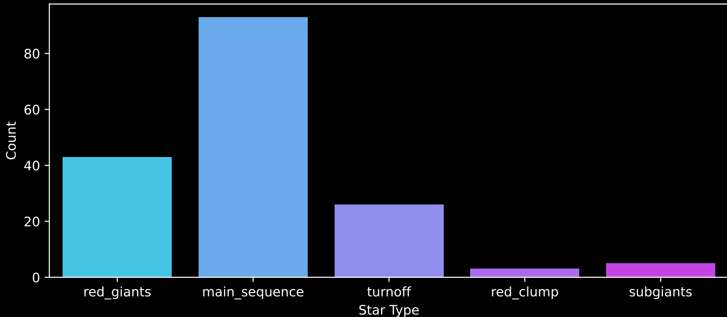
APOGEE DR17 Field: [047+39_MGA] Count plot of Star Type
